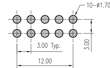
Recommended P.C.B. Layout Layout Tolerance = ± 0.05 mm
