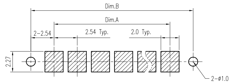
Recommended P.C.B. Layout Layout Tolerance = ± 0.05 mm
