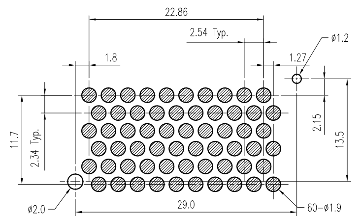
Recommended P.C.B. Layout Layout Tolerance = ± 0.05 mm
